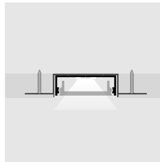
INCASSO CON CASSAFORMA RECESSED WITH FORMWORK CESTAL0095
