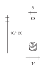
1497.30 _ 1x60W _ G9
