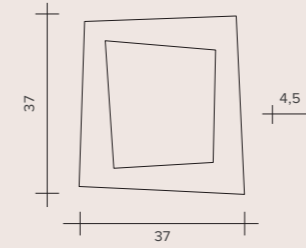
LED 18W - 300 mA 3000°K / 1440 lumen
