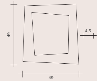
LED 30W - 300 mA 3000°K / 2400 lumen
