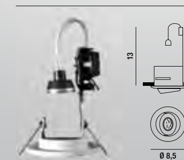
6128 CR Faretto da incasso orientabile in alluminio cromo spazzolato Aluminium recessed downlight adjustable brushed chrome
