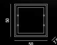
5746 ST Plafoniera vetro satinato Satin glass ceiling lamp
