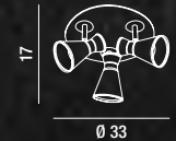
6136 B Plafoniera 3 luci in vetro bianco e trasparente White and transparent glass 3 lights ceiling lamp
