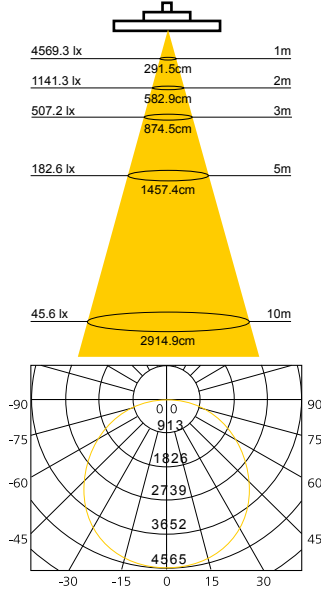
LD1HB100G - 120°
