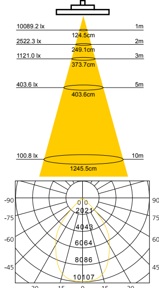
LD1HB100G - 60°
